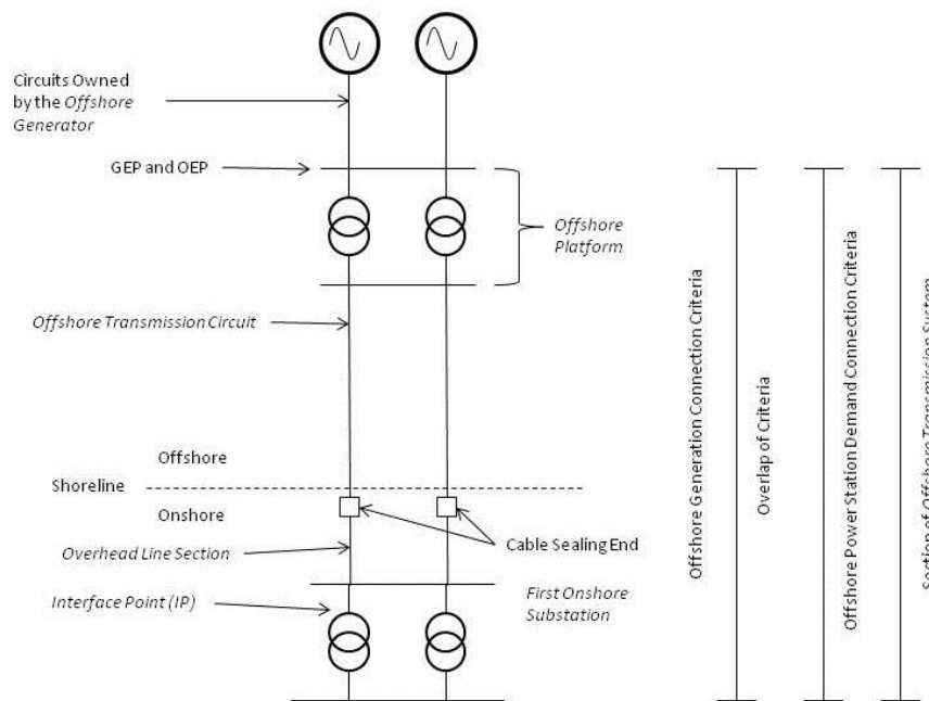
Figure 1.2 The offshore transmission system with a directly connected power station and first onshore substation
